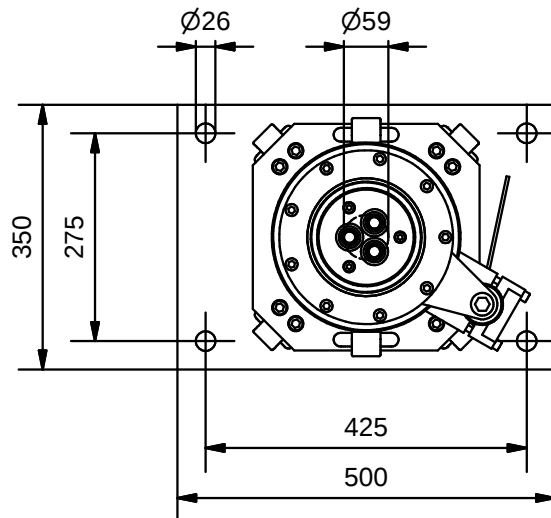
Top view (1:10)
